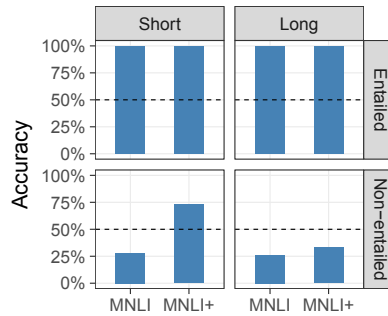
Figure 3: Results on the lexical overlap cases from Dasgupta et al. (2018) for BERT fine-tuned on MNLI or on MNLI augmented with HANS-like examples.
